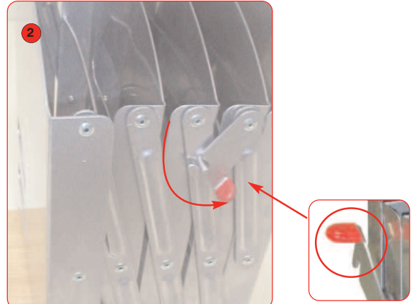
Push locking arm backwards to release
